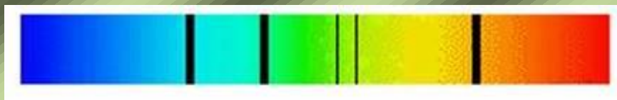
Cool star
